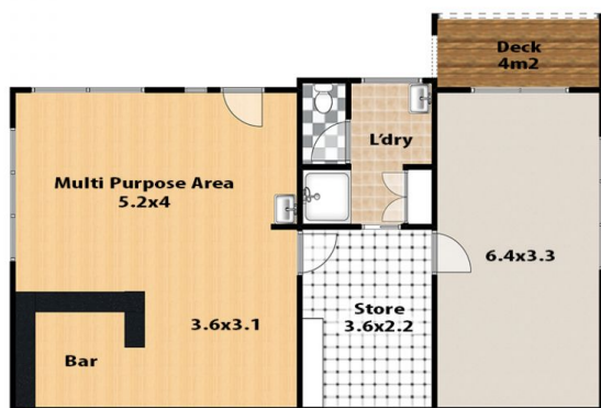
Lower Level
