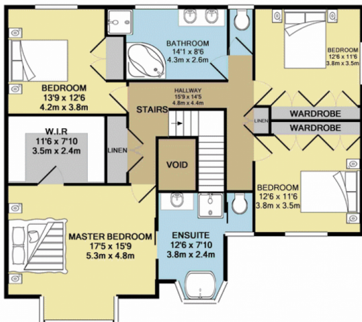
1ST FLOOR
