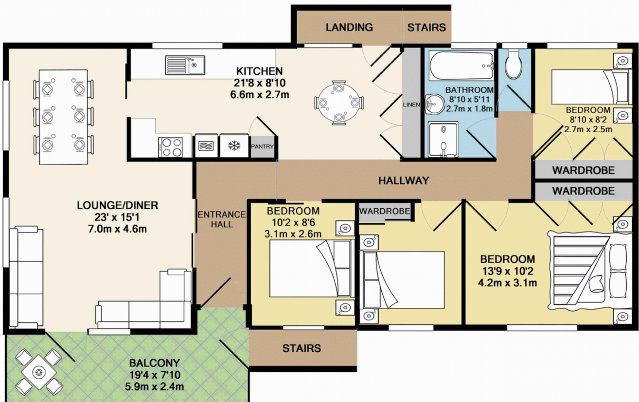
1ST FLOOR
