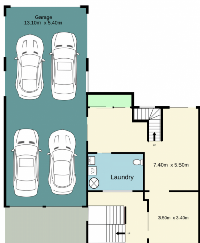
Ground floor 153.4 sq.m. approx.
