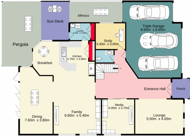
Ground floor 266.7 sq.m. approx.
