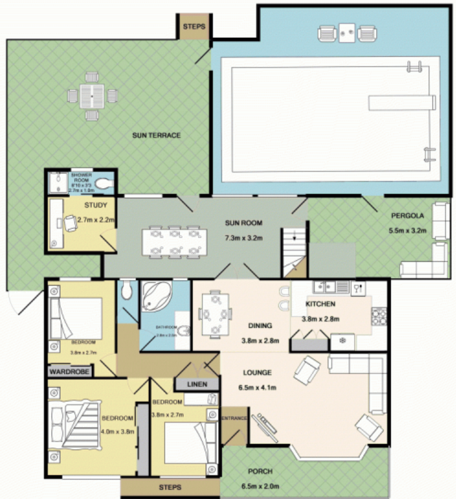
1ST FLOOR
